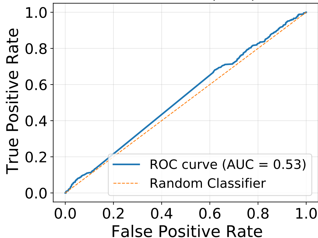
ROC Curve (Test)
